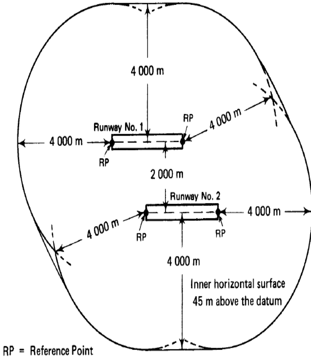
Inner Horizontal Surface for runway code 3 & 4
